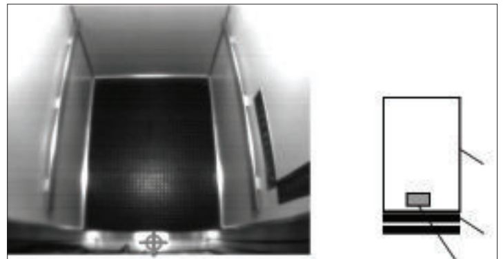
Figure 5: Correct mounting location for ESPROS/VOL-A on wall of elevator cab above elevator door
